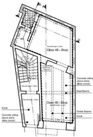
GROUND FLOOR PROPOSED (CLEAN COPY) SCALE 1:100
