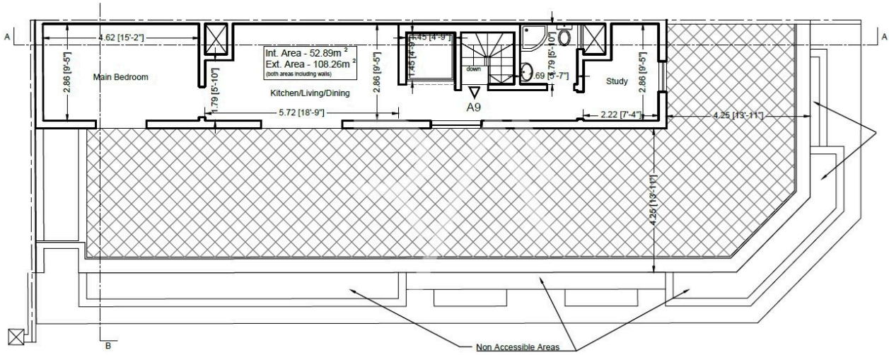
Receded Floor Level Scale 1:100
