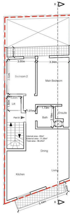
Proposed Third Floor Scale 1:100
