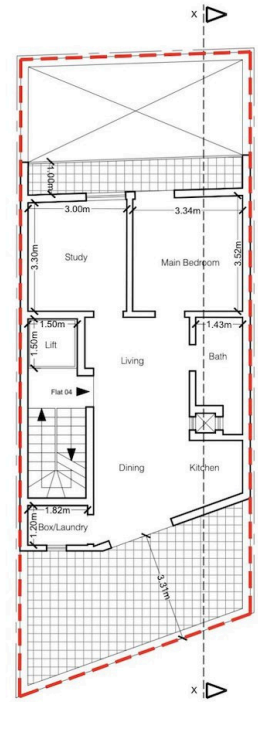
Proposed Receded Floor Scale 1:100
