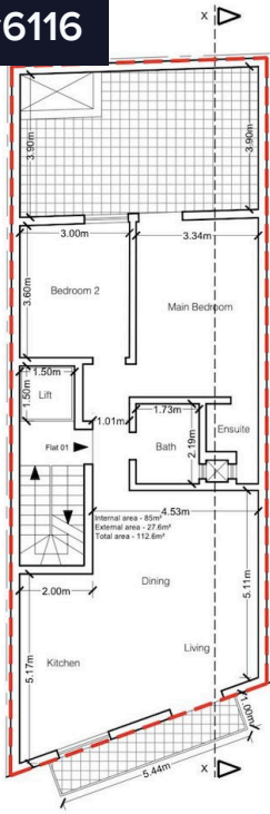
Proposed First Floor Scale 1:100
