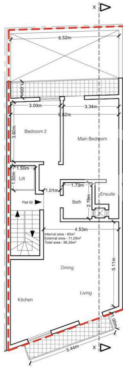
Proposed Second Floor Scale 1:100
