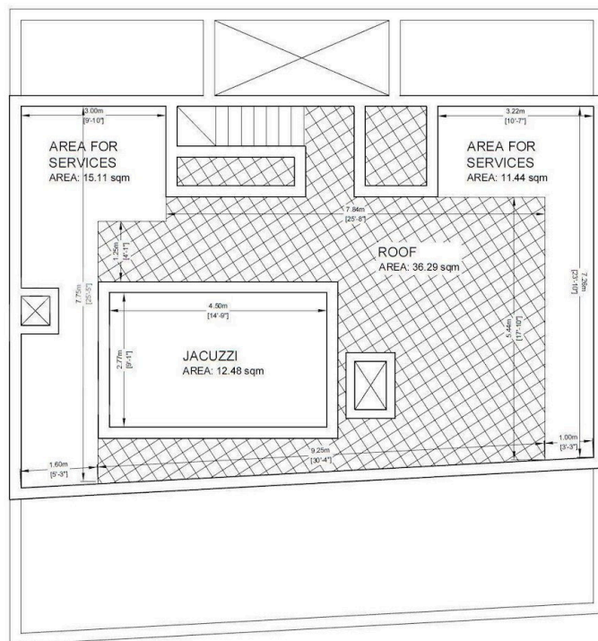
PROPOSED ROOF LEVEL SCALE 1:100
